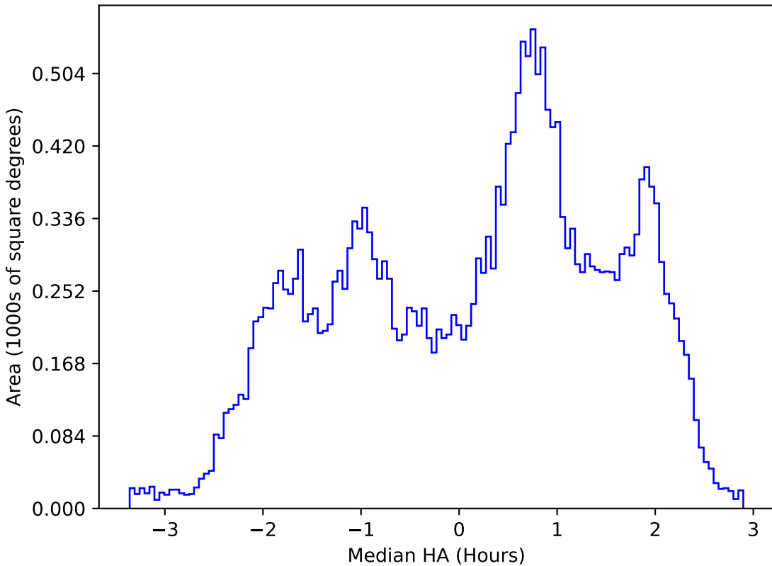
weather_cloudso31v3.4_10yrs All sky g band: Median HA
