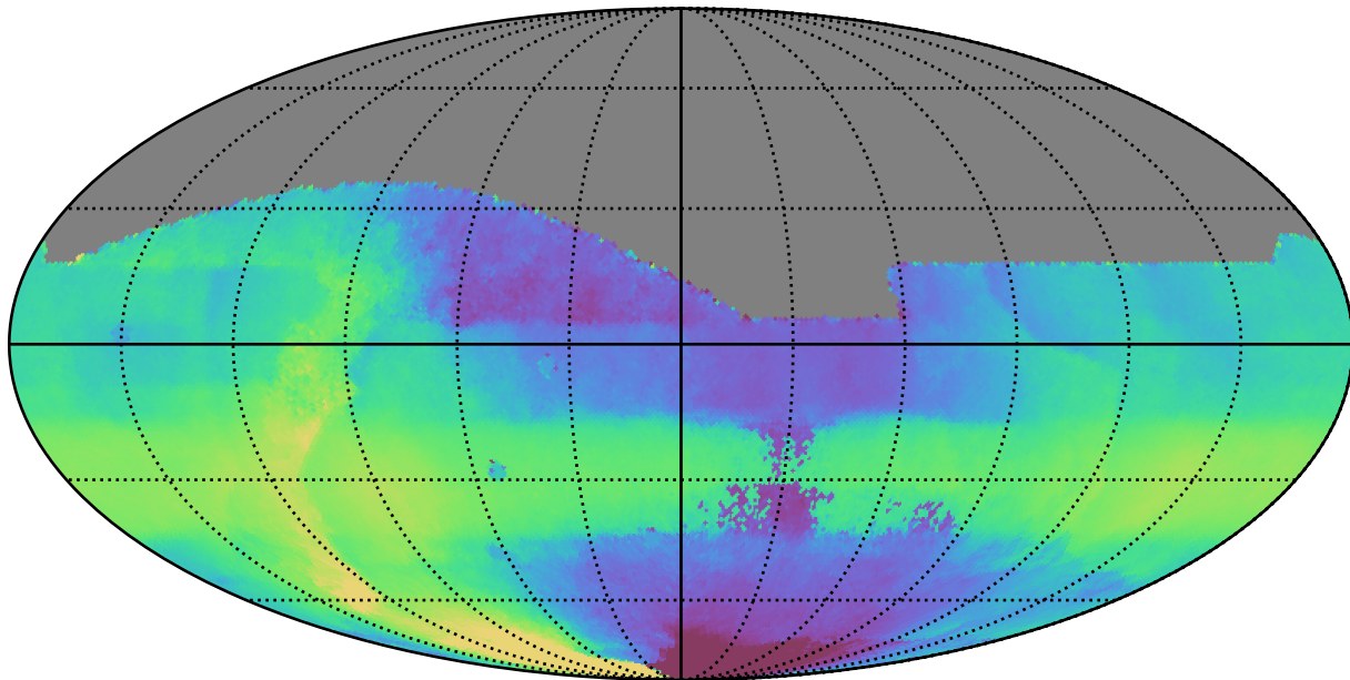
weather_cloudso31v3.4_10yrs All sky all bands: Median HA
