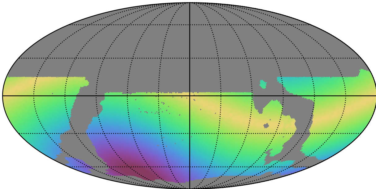
weather_cloudso31v3.4_10yrs WFD z band: Max solarElong
