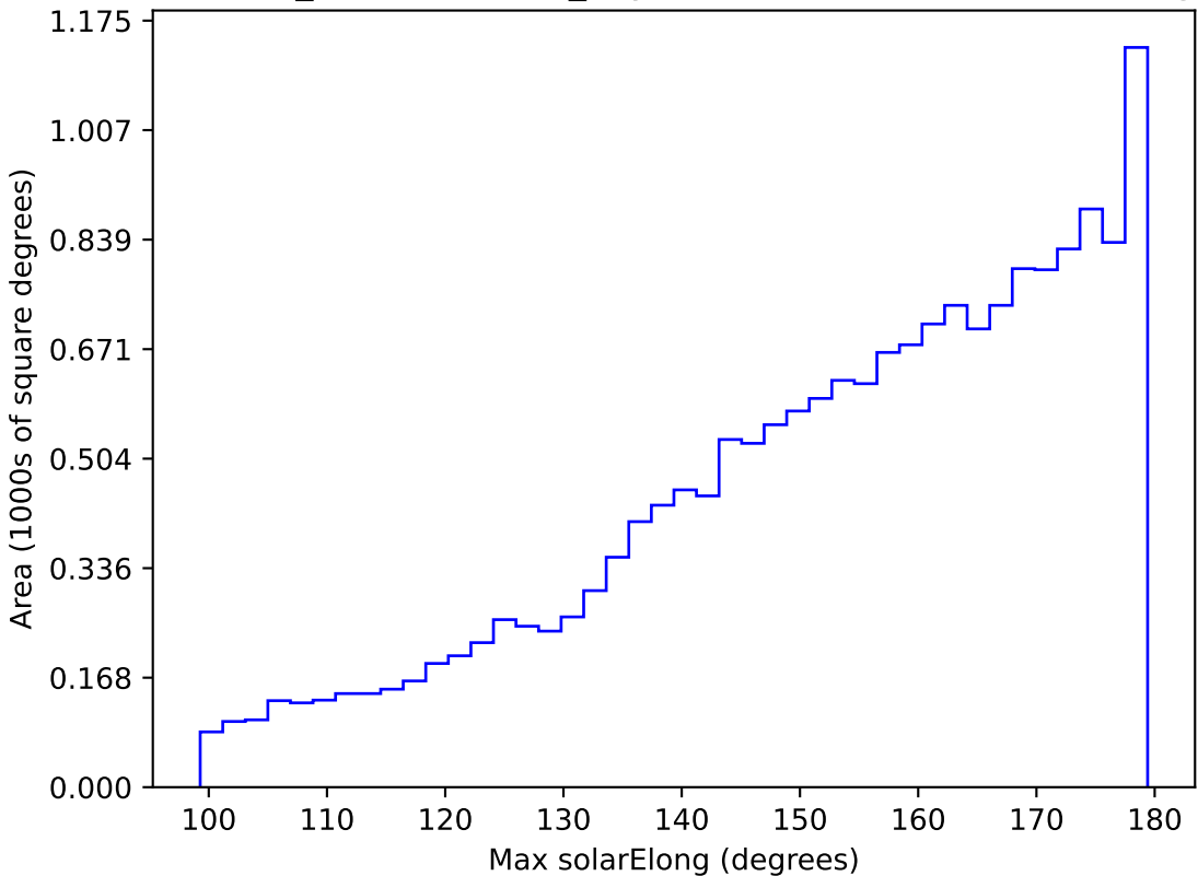
weather_cloudso31v3.4_10yrs WFD z band: Max solarElong
