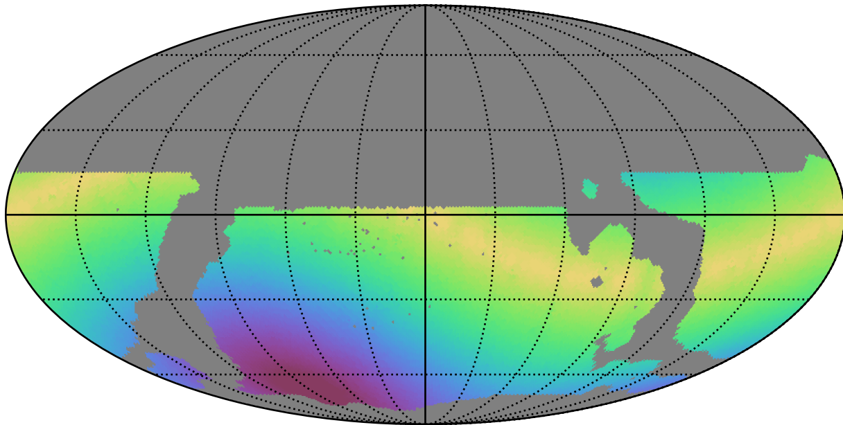
weather_cloudso31v3.4_10yrs WFD u band: Max solarElong
