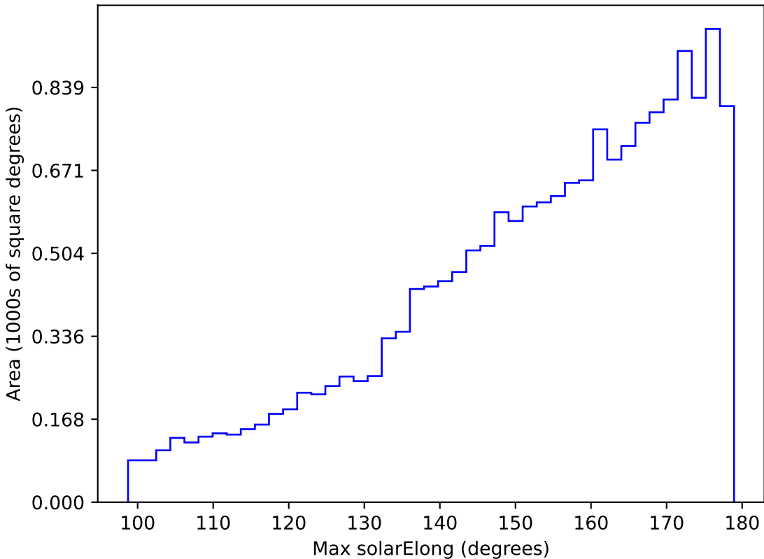
weather_cloudso31v3.4_10yrs WFD u band: Max solarElong
