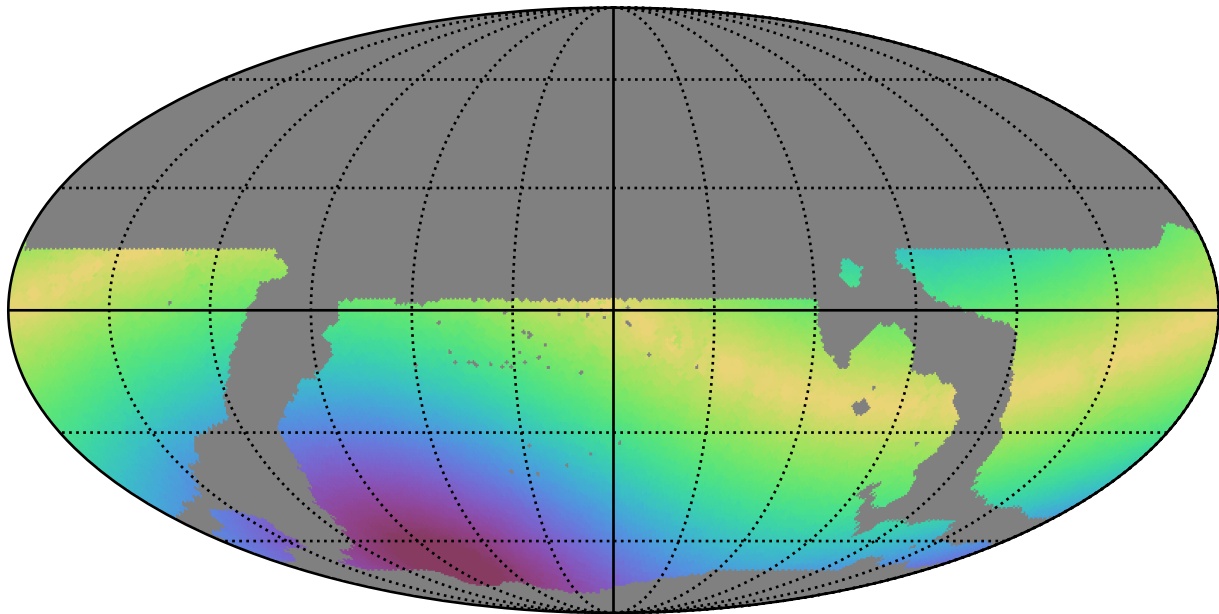
weather_cloudso31v3.4_10yrs WFD g band: Max solarElong
