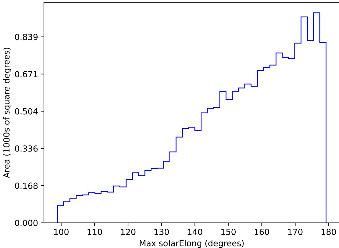
weather_cloudso31v3.4_10yrs WFD g band: Max solarElong
