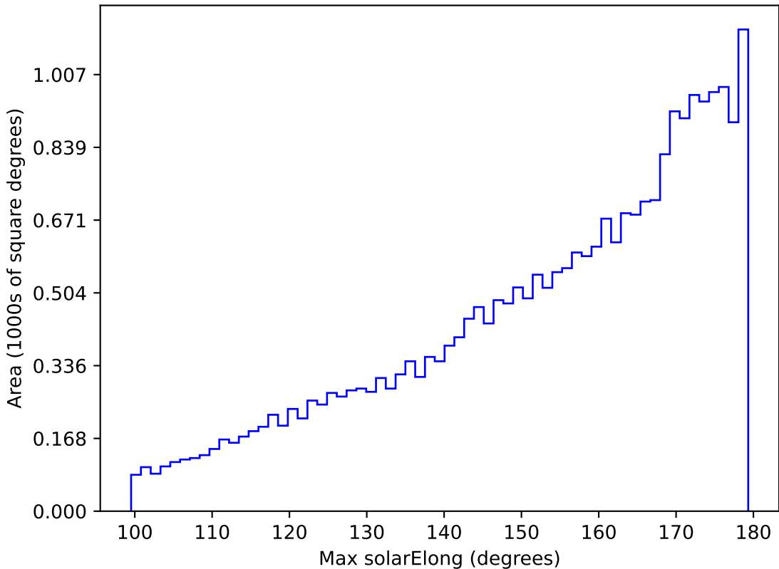
weather_cloudso31v3.4_10yrs All sky z band: Max solarElong
