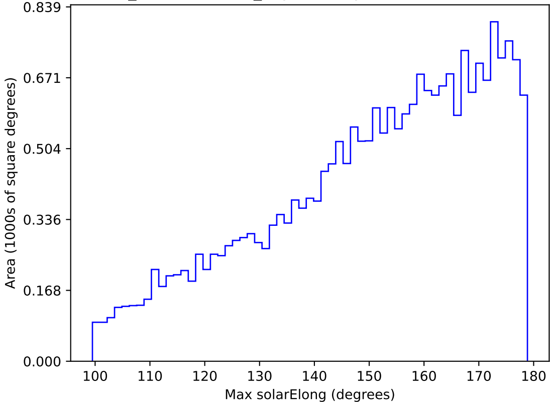
weather_cloudso31v3.4_10yrs All sky u band: Max solarElong
