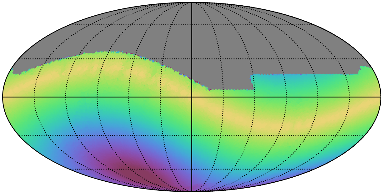
weather_cloudso31v3.4_10yrs All sky r band: Max solarElong
