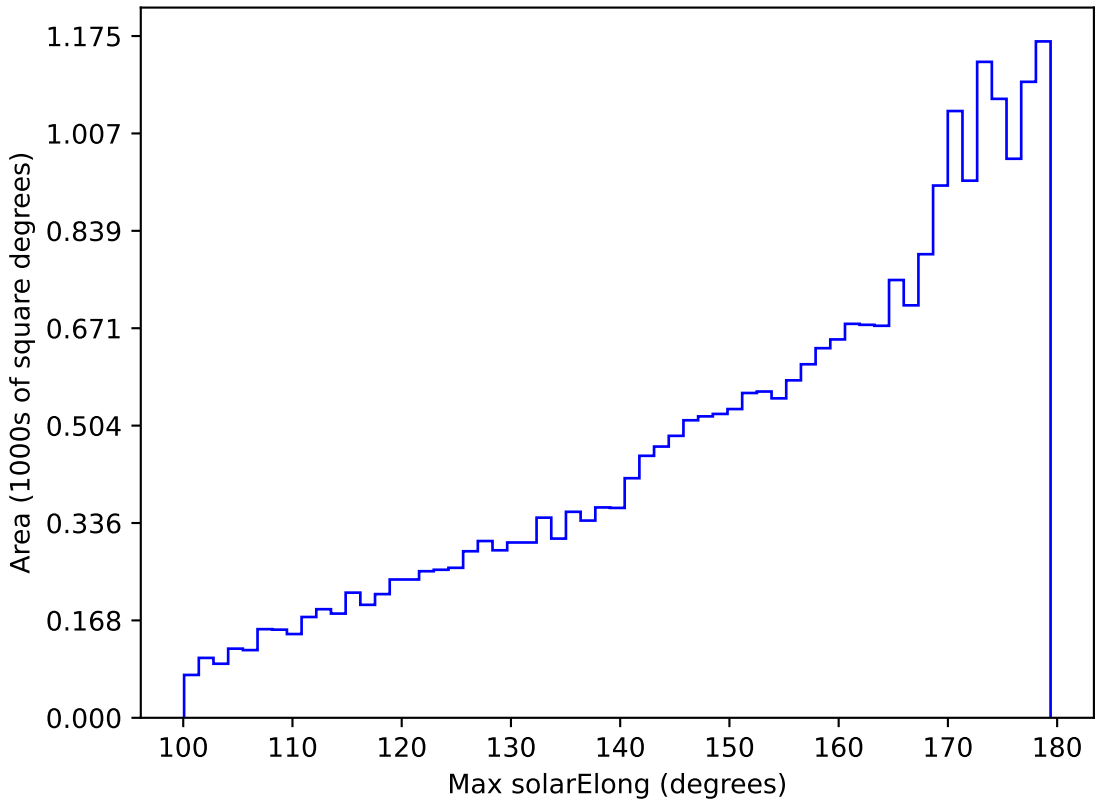
weather_cloudso31v3.4_10yrs All sky r band: Max solarElong
