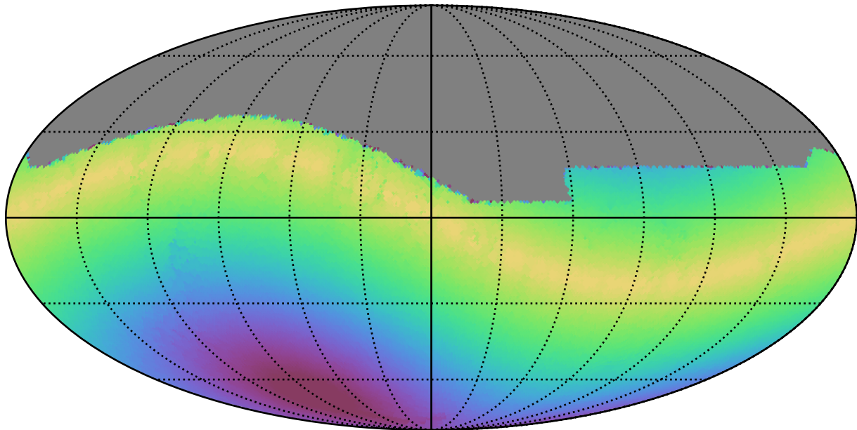
weather_cloudso31v3.4_10yrs All sky g band: Max solarElong
