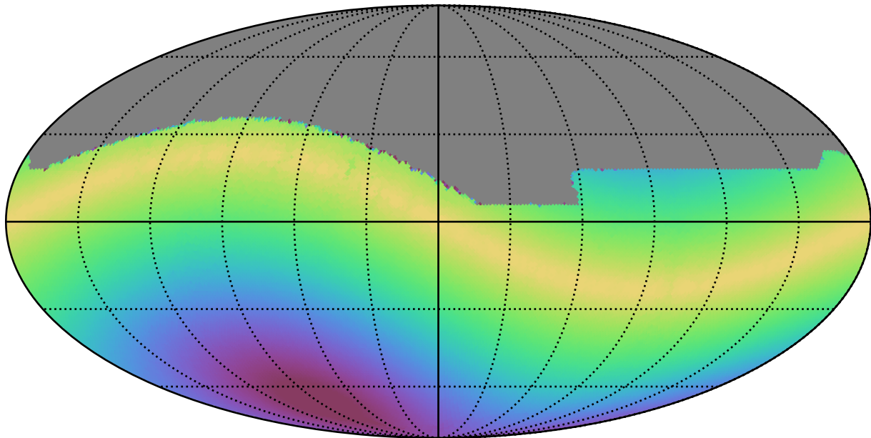
weather_cloudso31v3.4_10yrs All sky all bands: Max solarElong
