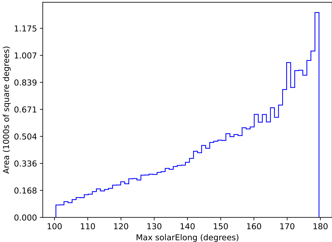
weather_cloudso31v3.4_10yrs All sky all bands: Max solarElong
