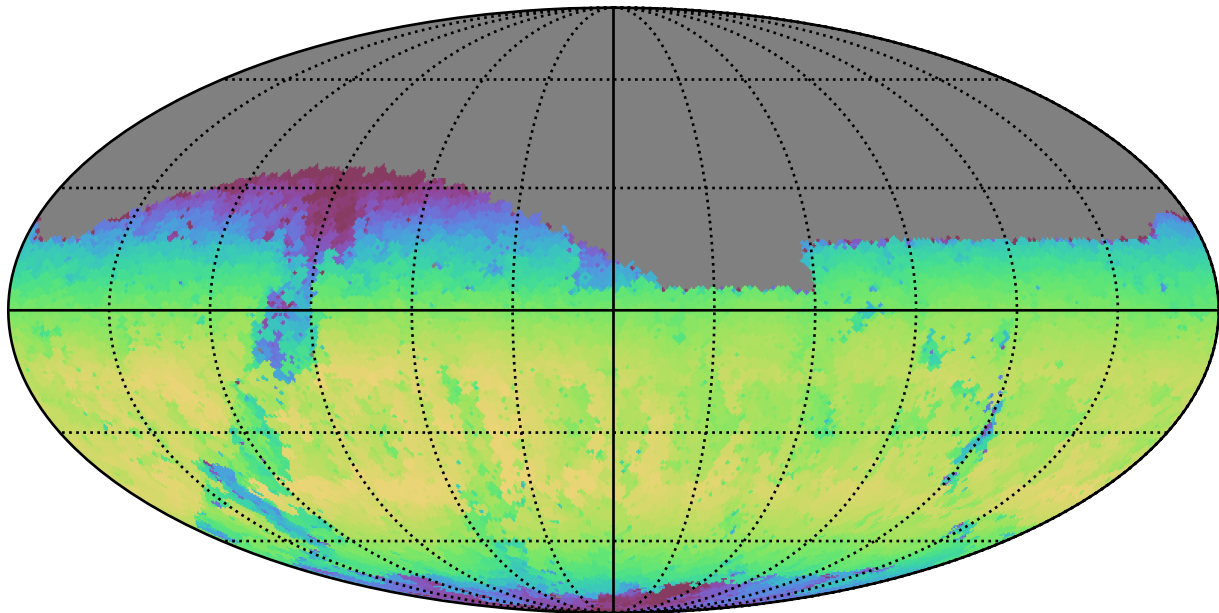
weather_cloudso31v3.4_10yrs Yr 1 z band: Max skyBrightness
