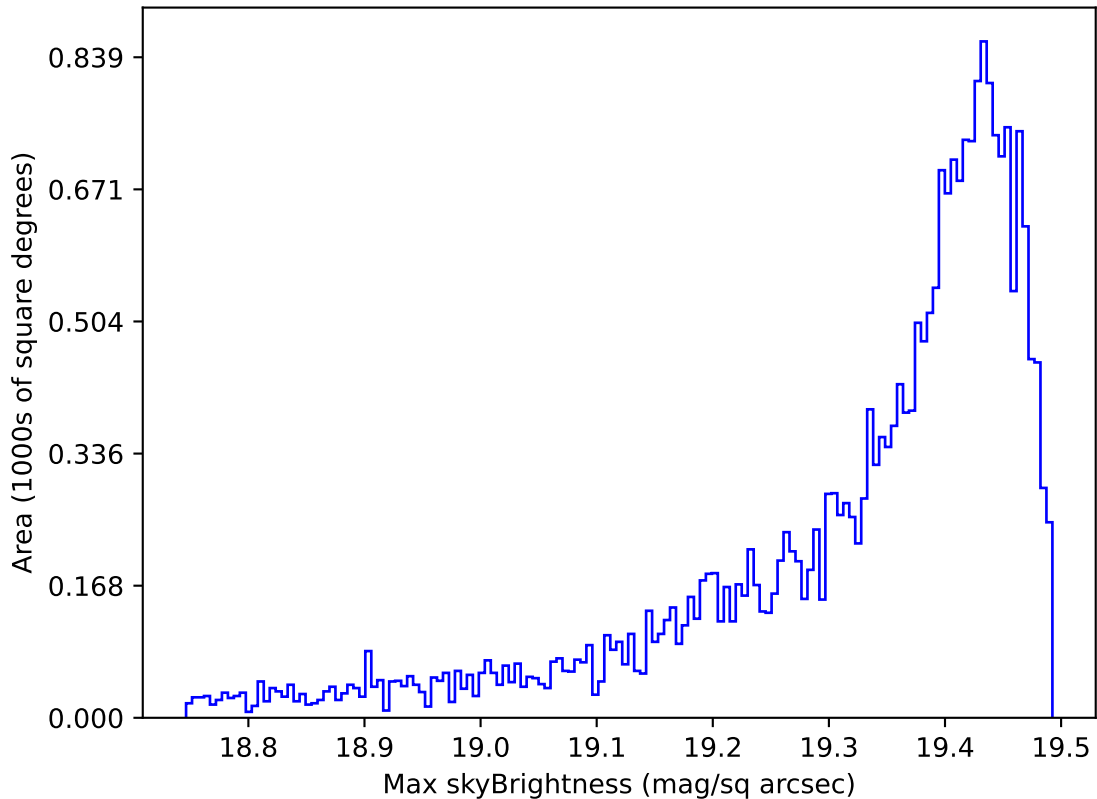
weather_cloudso31v3.4_10yrs Yr 1 z band: Max skyBrightness
