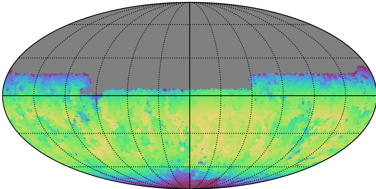
weather_cloudso31v3.4_10yrs Yr 1 y band: Max skyBrightness
