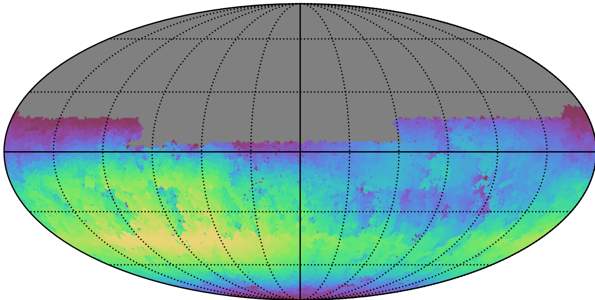
weather_cloudso31v3.4_10yrs Yr 1 u band: Max skyBrightness
