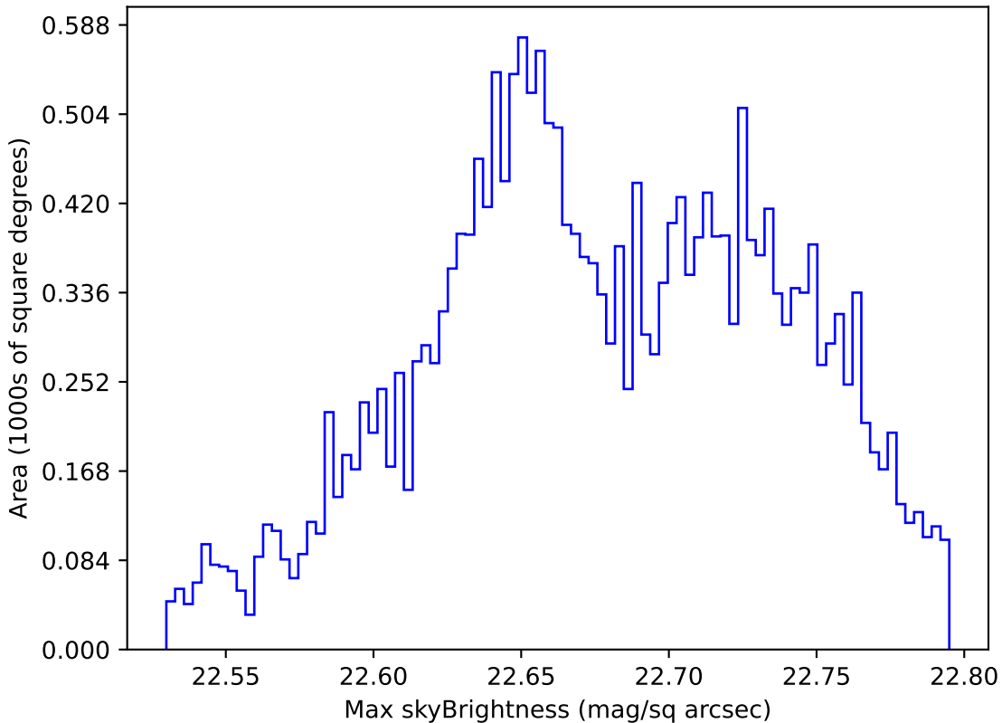
weather_cloudso31v3.4_10yrs Yr 1 u band: Max skyBrightness
