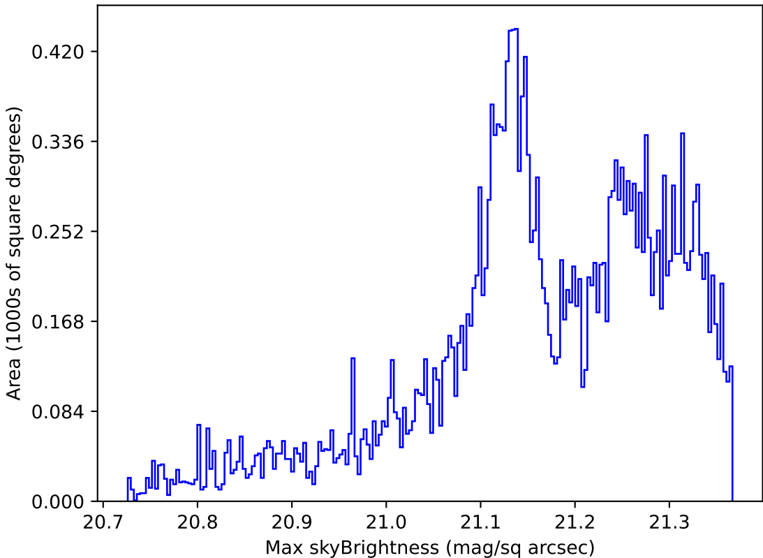
weather_cloudso31v3.4_10yrs Yr 1 r band: Max skyBrightness
