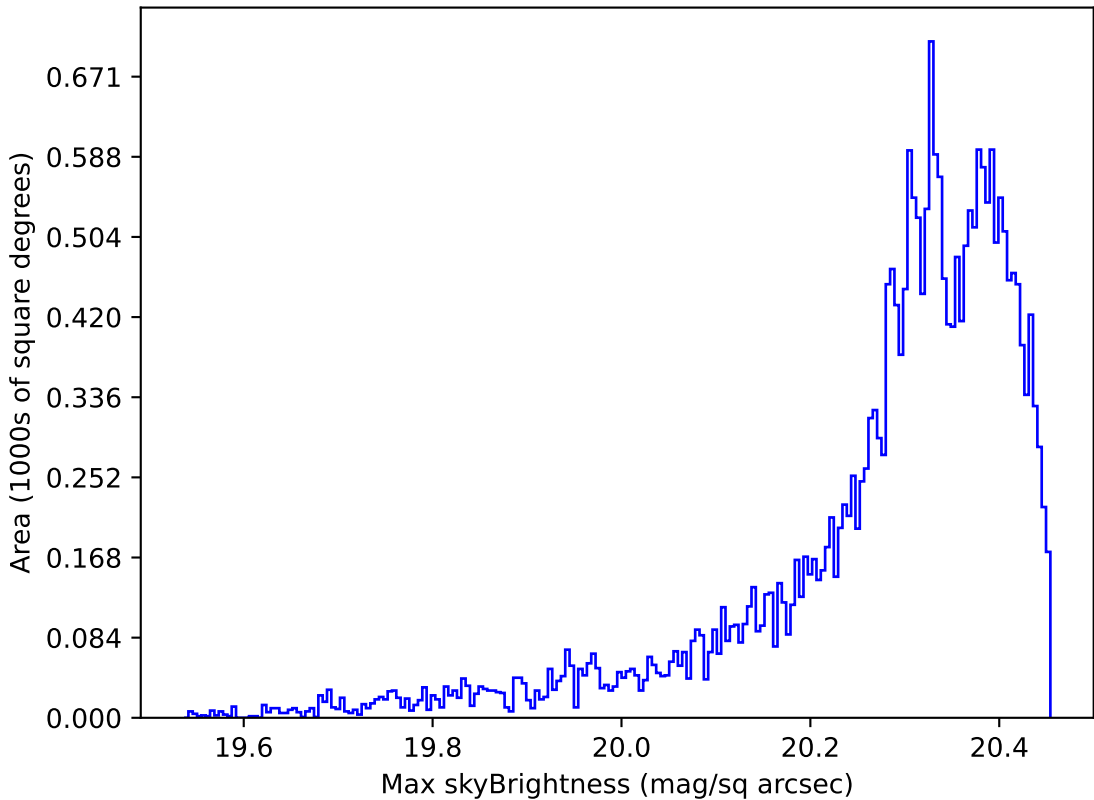
weather_cloudso31v3.4_10yrs Yr 1 i band: Max skyBrightness
