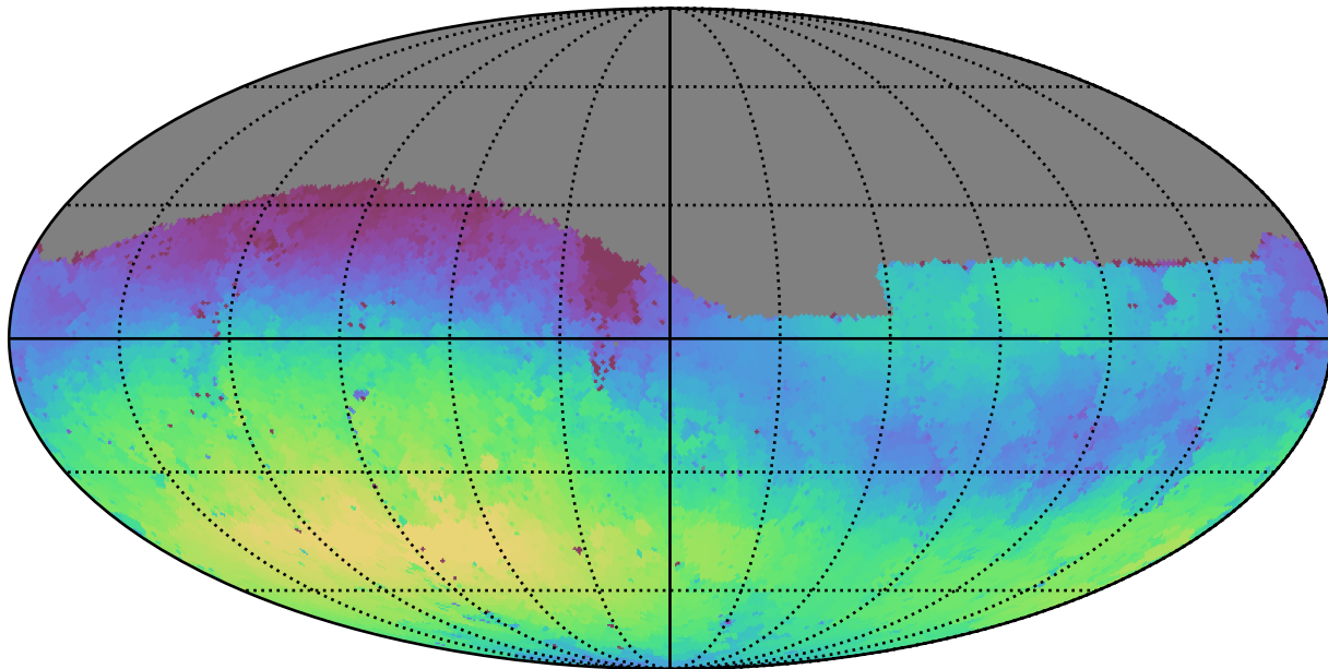
weather_cloudso31v3.4_10yrs Yr 1 g band: Max skyBrightness
