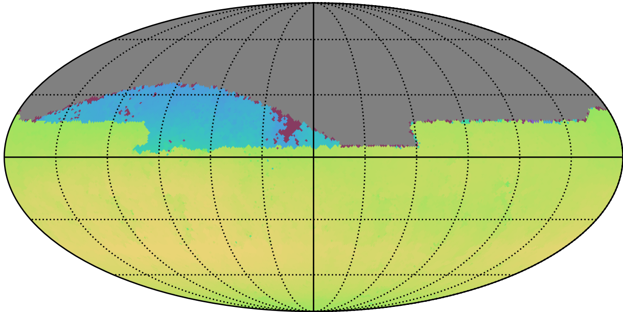
weather_cloudso31v3.4_10yrs Yr 1 all bands: Max skyBrightness
