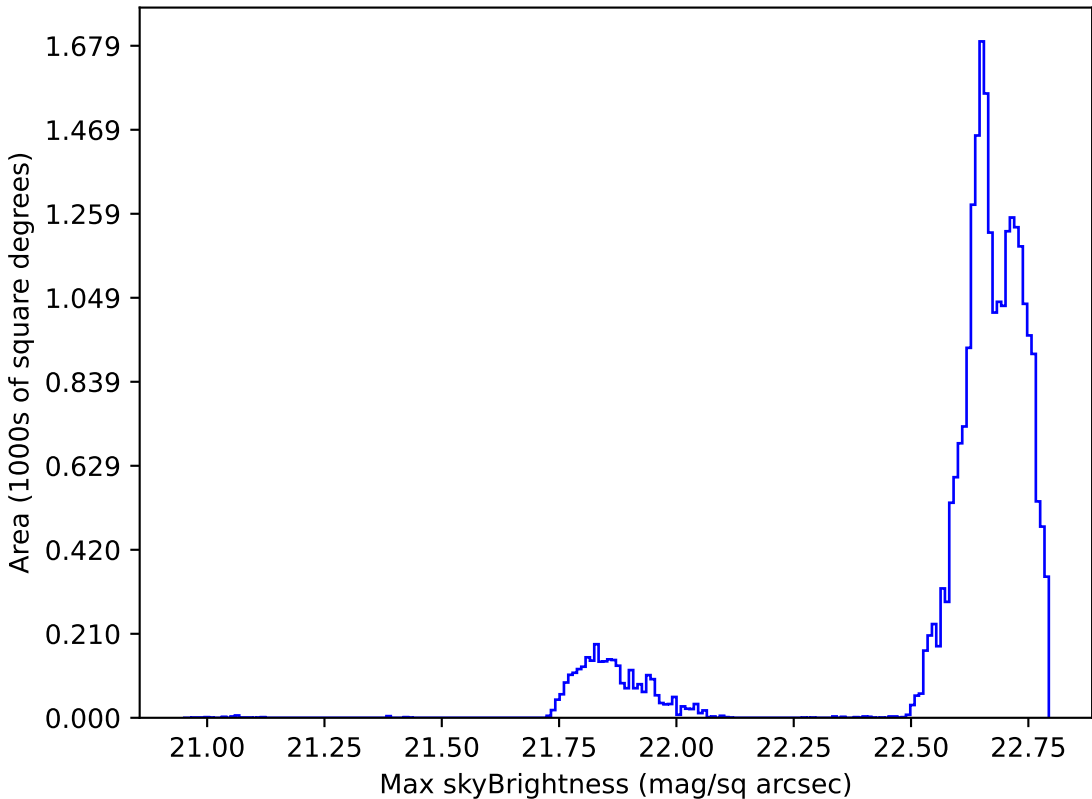
weather_cloudso31v3.4_10yrs Yr 1 all bands: Max skyBrightness
