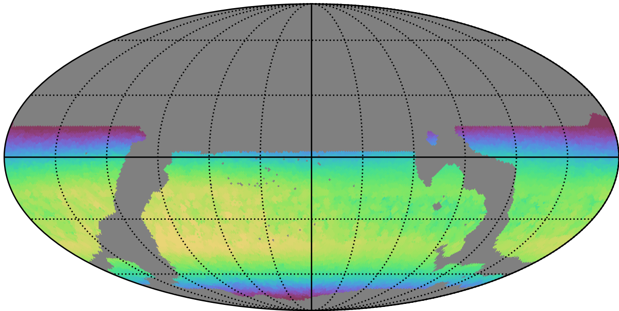
weather_cloudso31v3.4_10yrs WFD z band: Max skyBrightness
