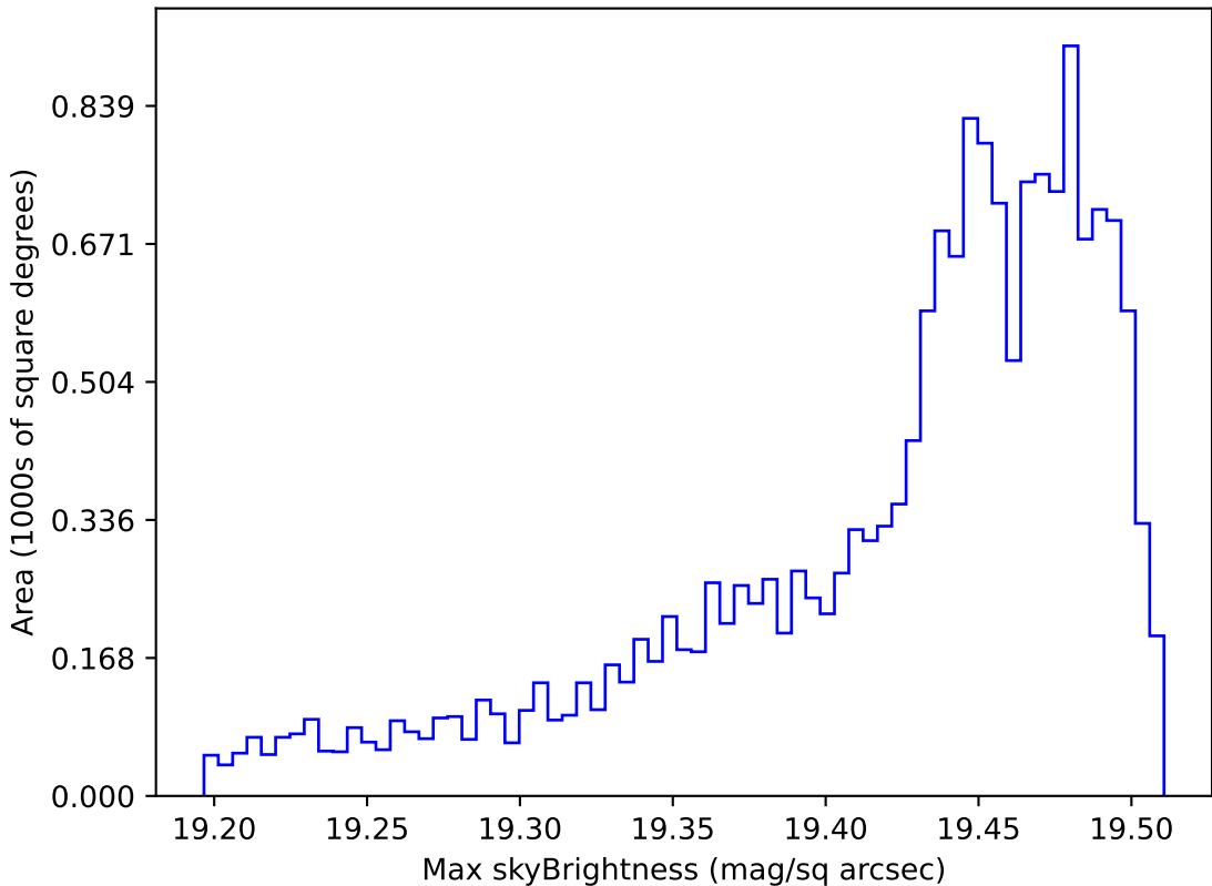
weather_cloudso31v3.4_10yrs WFD z band: Max skyBrightness
