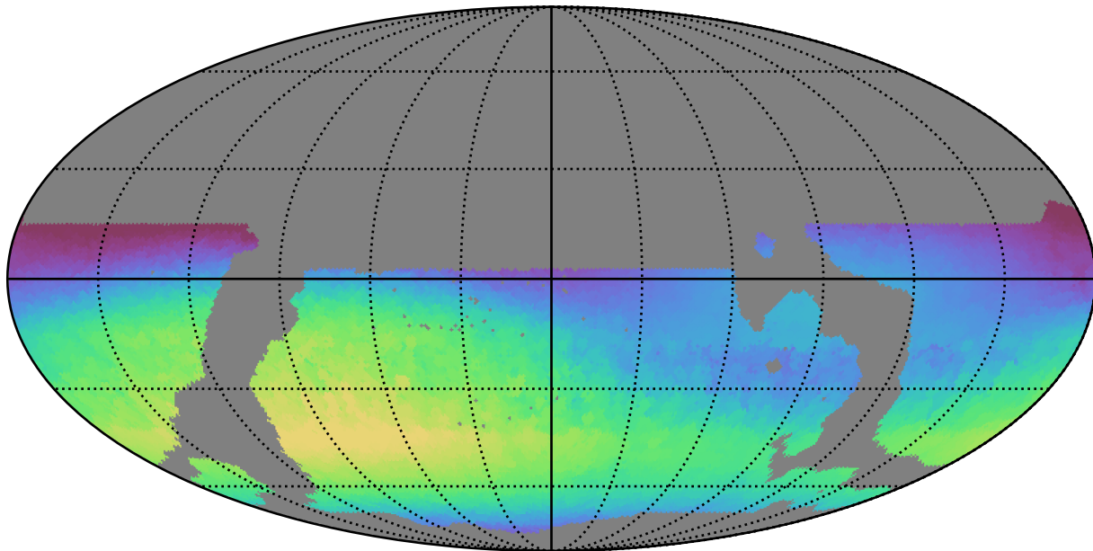
weather_cloudso31v3.4_10yrs WFD u band: Max skyBrightness
