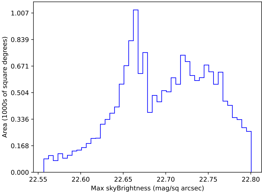
weather_cloudso31v3.4_10yrs WFD u band: Max skyBrightness
