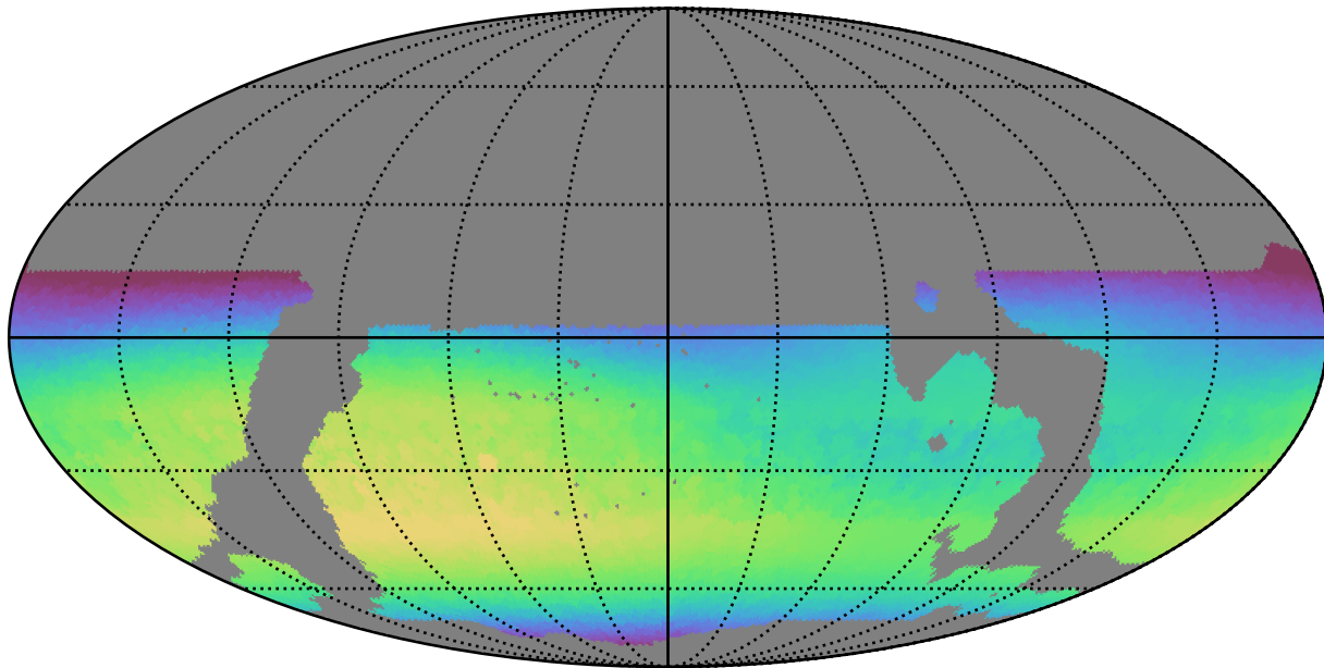
weather_cloudso31v3.4_10yrs WFD i band: Max skyBrightness
