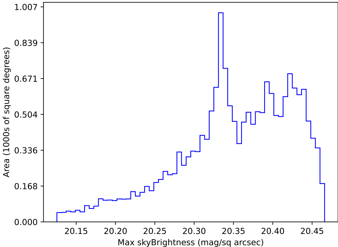
weather_cloudso31v3.4_10yrs WFD i band: Max skyBrightness
