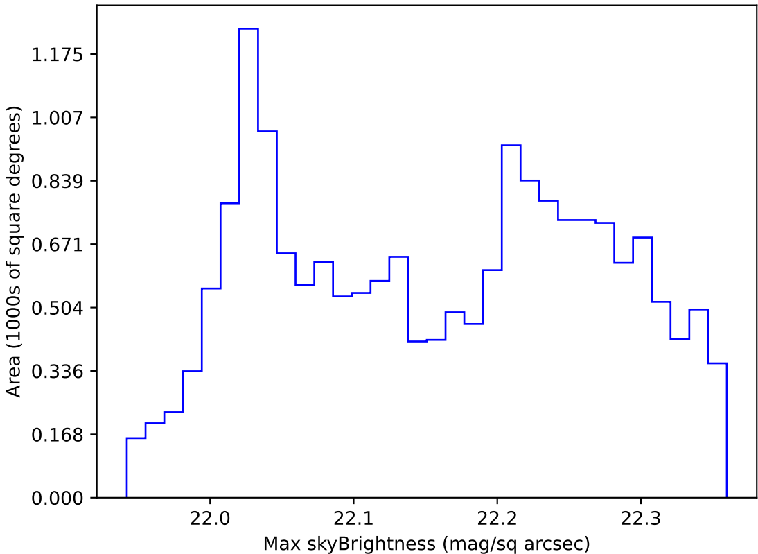
weather_cloudso31v3.4_10yrs WFD g band: Max skyBrightness
