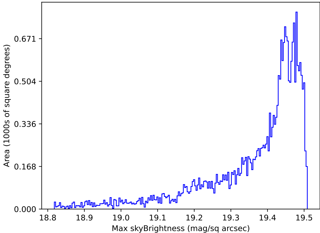
weather_cloudso31v3.4_10yrs All sky z band: Max skyBrightness
