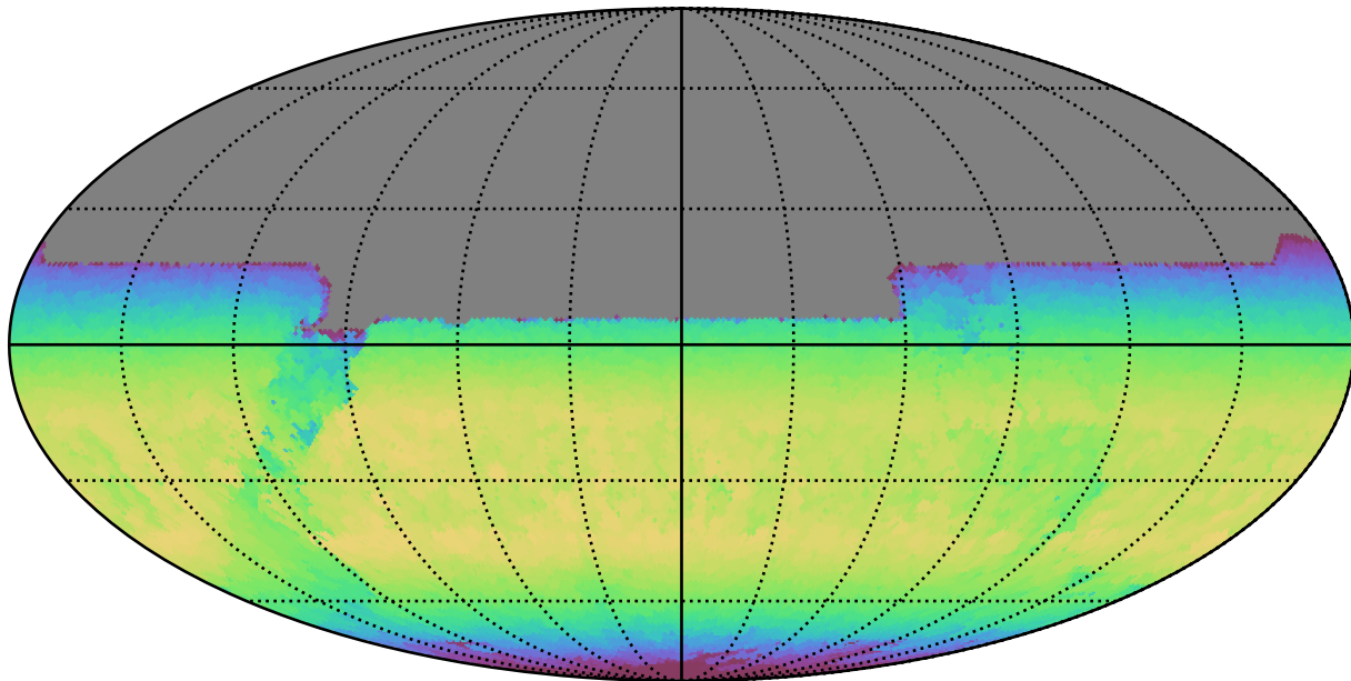
weather_cloudso31v3.4_10yrs All sky y band: Max skyBrightness
