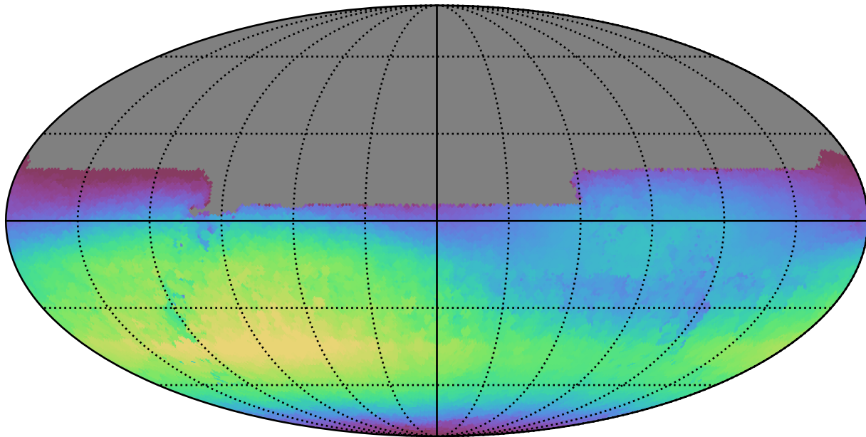
weather_cloudso31v3.4_10yrs All sky u band: Max skyBrightness
