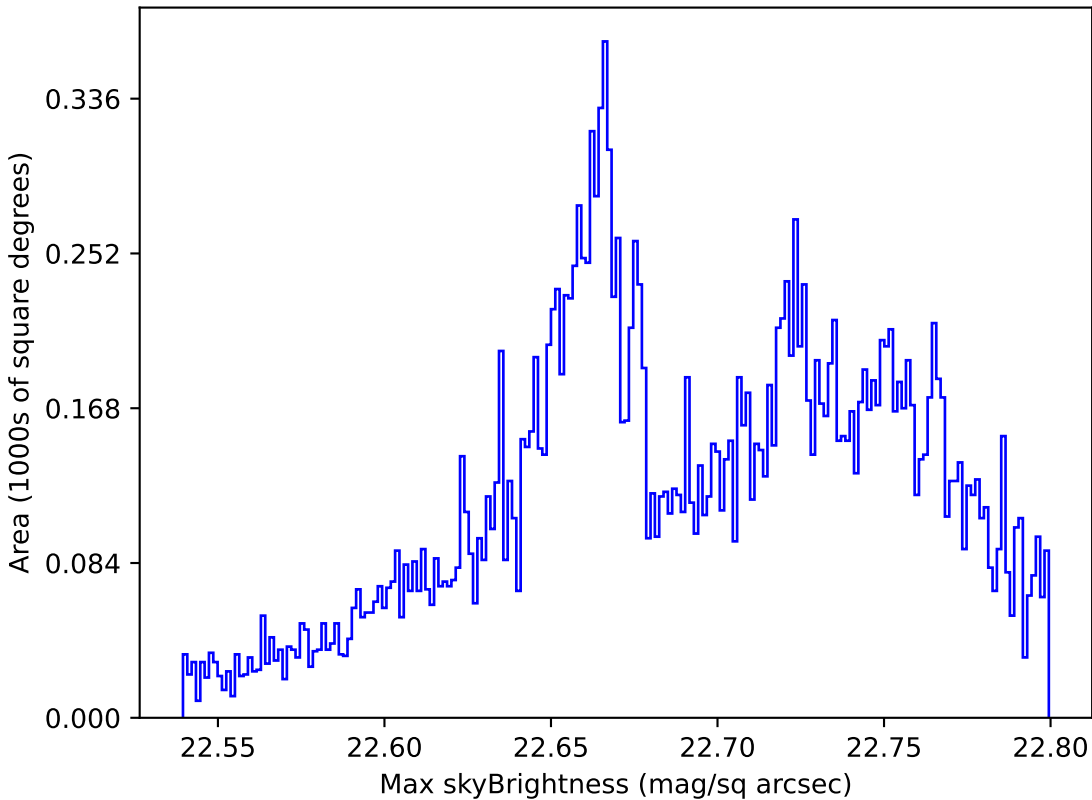
weather_cloudso31v3.4_10yrs All sky u band: Max skyBrightness
