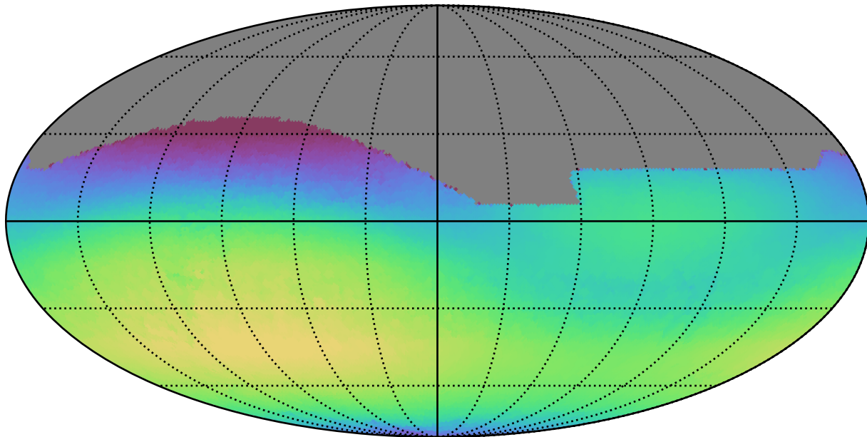
weather_cloudso31v3.4_10yrs All sky r band: Max skyBrightness
