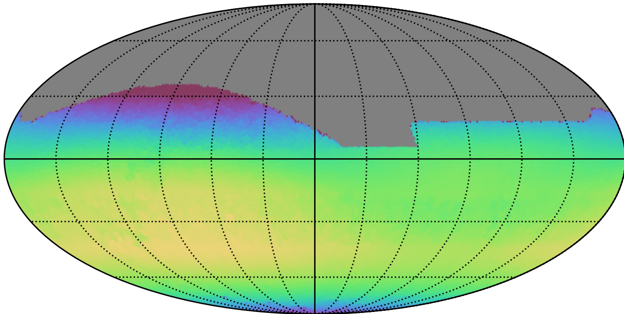
weather_cloudso31v3.4_10yrs All sky i band: Max skyBrightness
