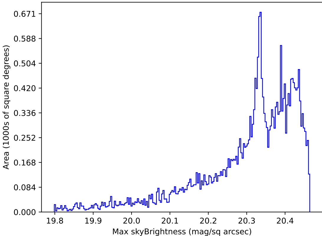
weather_cloudso31v3.4_10yrs All sky i band: Max skyBrightness
