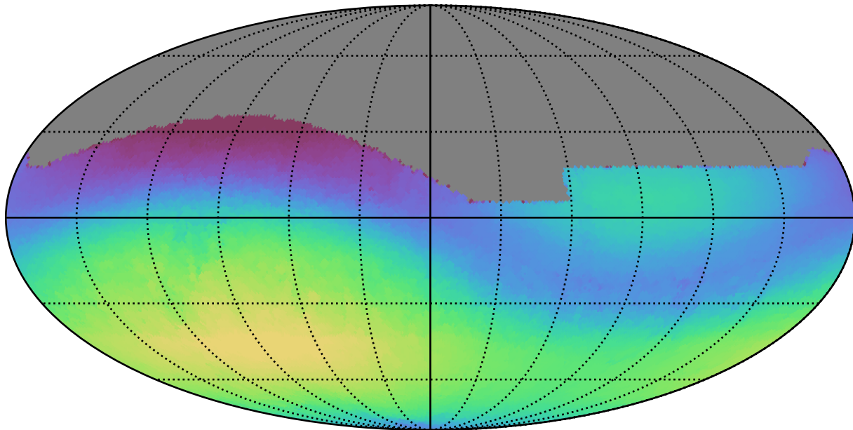
weather_cloudso31v3.4_10yrs All sky g band: Max skyBrightness
