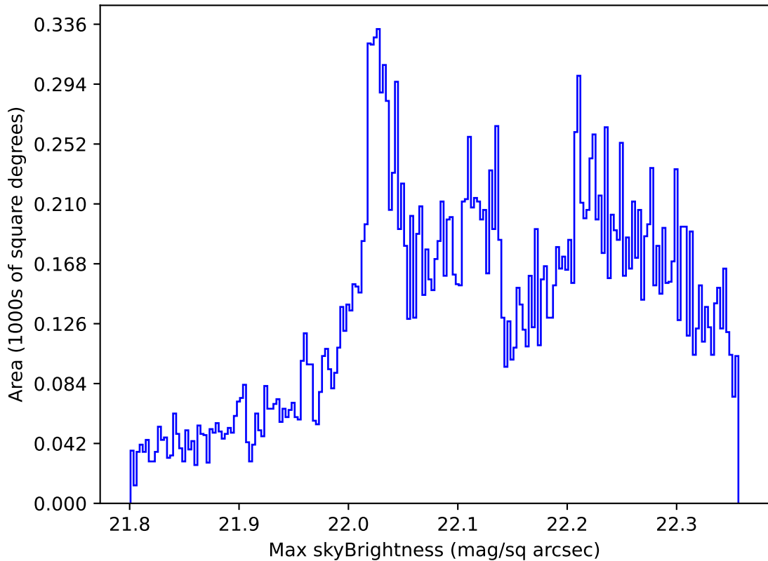
weather_cloudso31v3.4_10yrs All sky g band: Max skyBrightness
