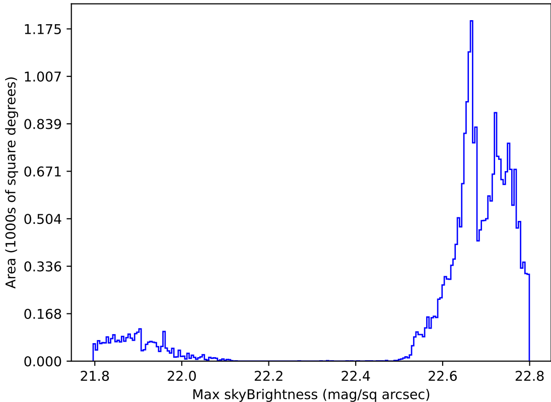
weather_cloudso31v3.4_10yrs All sky all bands: Max skyBrightness
