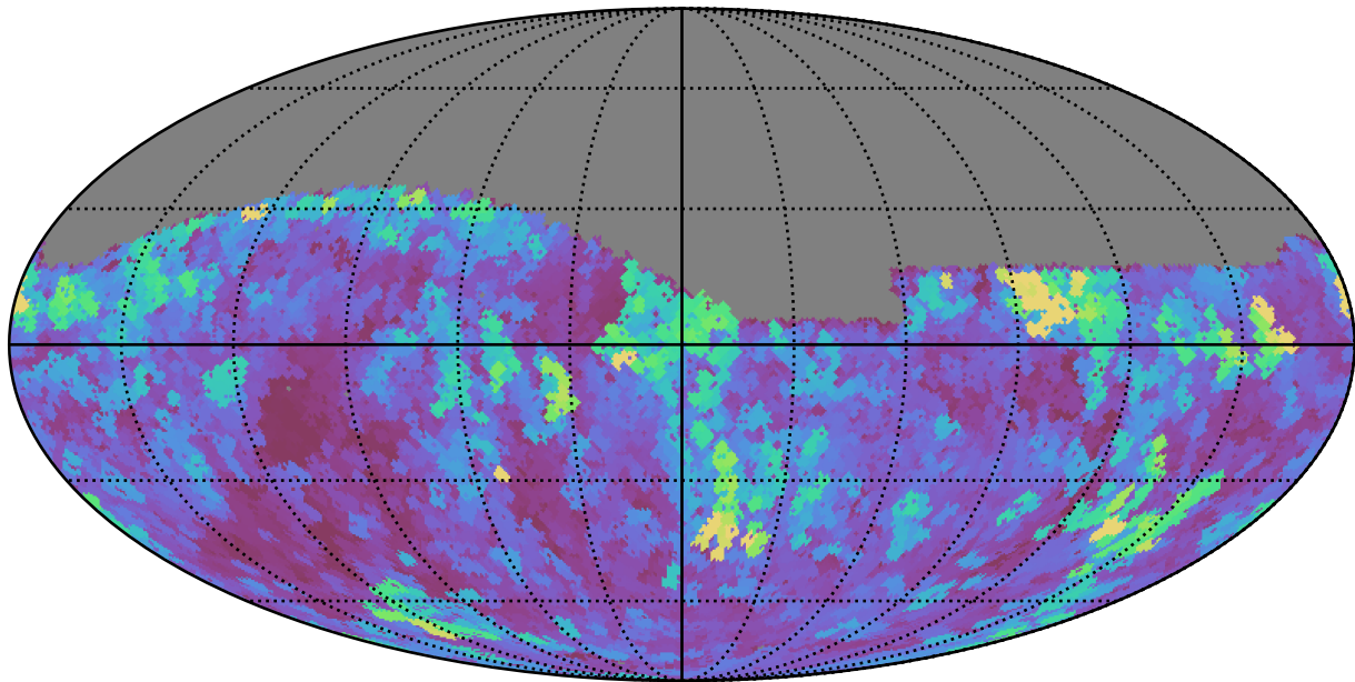
weather_cloudso31v3.4_10yrs Yr 1 z band: Max seeingGeom
