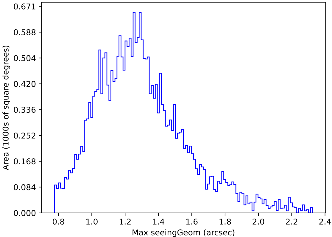
weather_cloudso31v3.4_10yrs Yr 1 r band: Max seeingGeom
