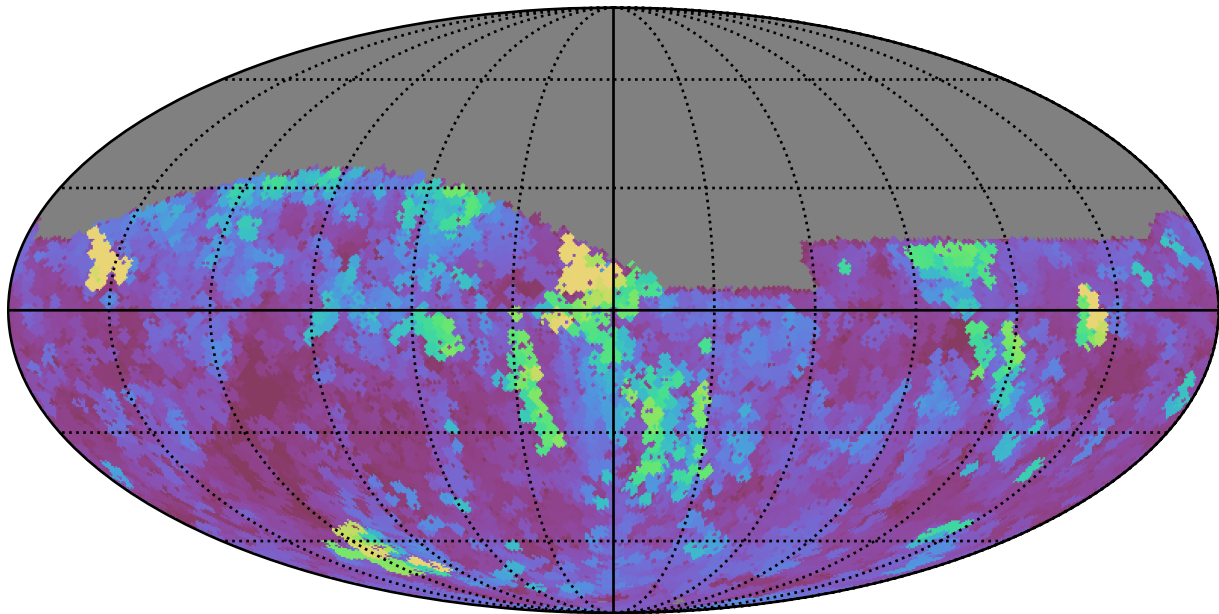
weather_cloudso31v3.4_10yrs Yr 1 i band: Max seeingGeom
