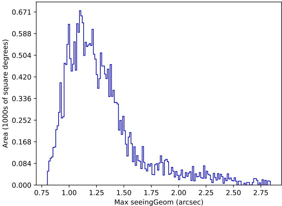
weather_cloudso31v3.4_10yrs Yr 1 i band: Max seeingGeom
