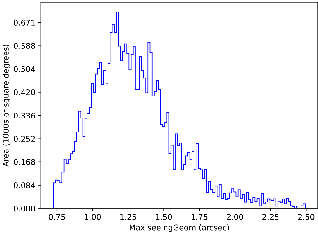
weather_cloudso31v3.4_10yrs Yr 1 g band: Max seeingGeom
