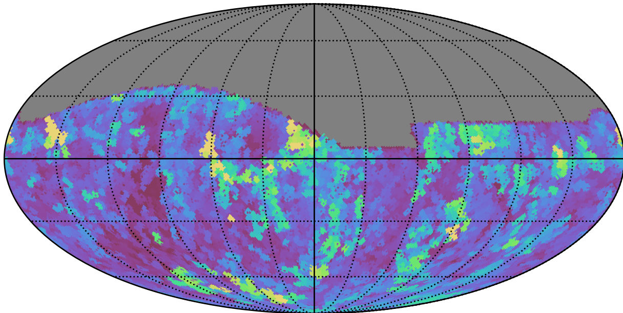
weather_cloudso31v3.4_10yrs Yr 1 all bands: Max seeingGeom
