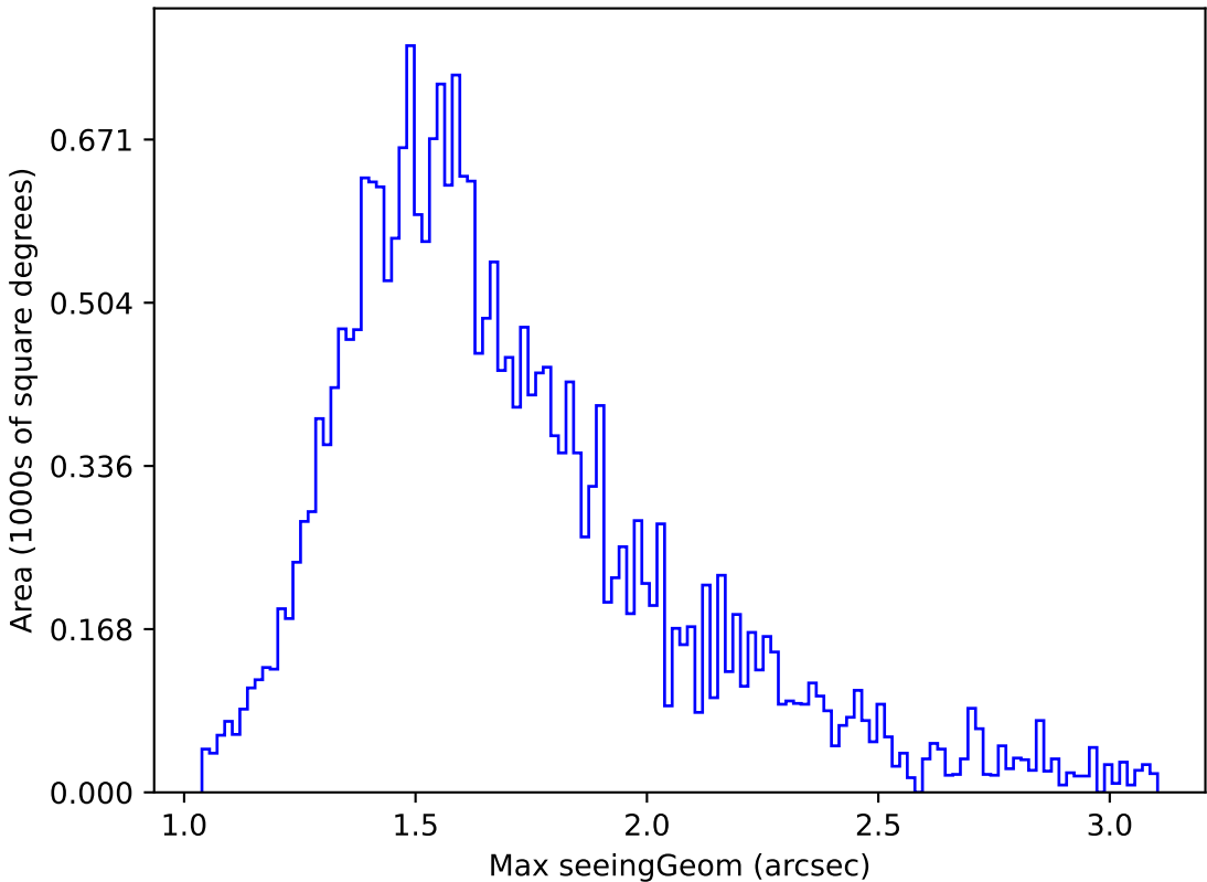
weather_cloudso31v3.4_10yrs Yr 1 all bands: Max seeingGeom
