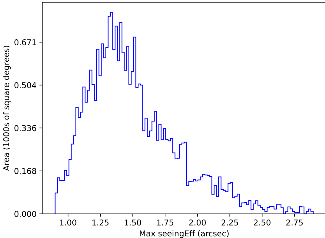
weather_cloudso31v3.4_10yrs Yr 1 z band: Max seeingEff
